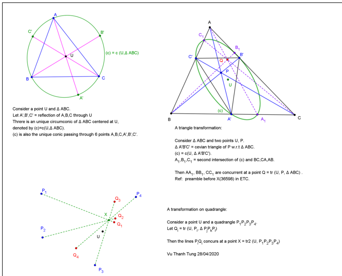
QuadrangleTransformation1.pdf
