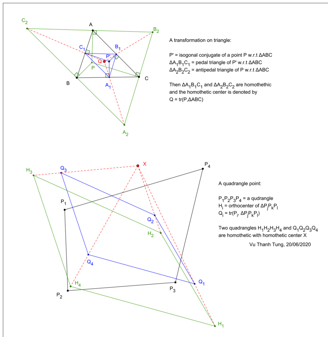
QA-HomotheticPoint2.pdf
