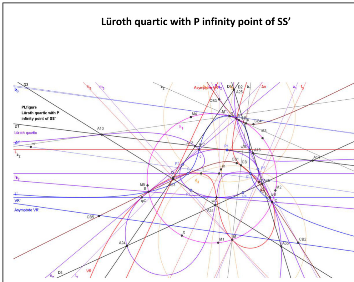
Lroth quartic with P infinity point of SS_.pdf
