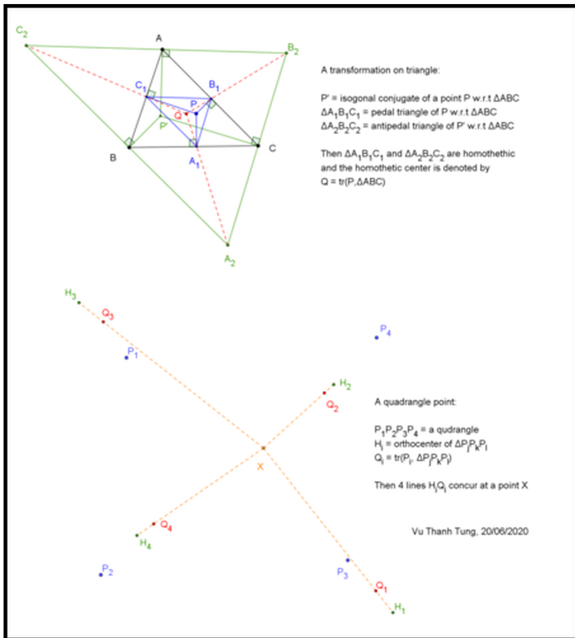
QA-HomotheticPoint22.png
